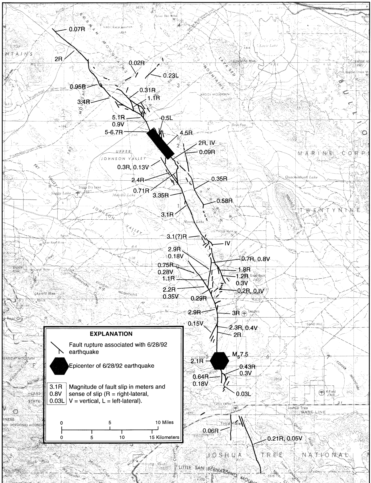
Figure 2. Surface faulting associated with the 1992 Landers earthquake. For details of shaded area, see Irvine and Hill, this issue.
